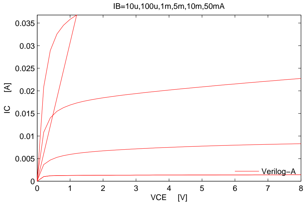
FIGURE 38. Forced-IB output characteristics at T=300K .
