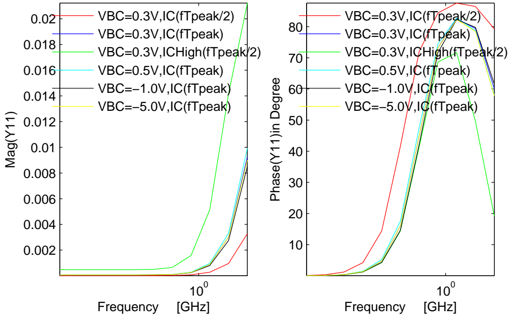
FIGURE 45. Y11 vs Frequency(GHz) plots at T=300K, Vbc=0.3, 0.5, -1.0 and -5.0V for IC(fTpeak),IC(ftpeak/2)and ICHigh(fTpeak/2).
