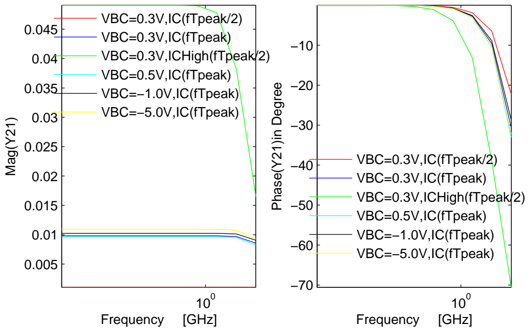
FIGURE 46. Y21 vs Frequency(GHz) plots at T=300K, Vbc=0.3, 0.5, -1.0 and -5.0V for IC(fTpeak),IC(ftpeak/2)and ICHigh(fTpeak/2).
