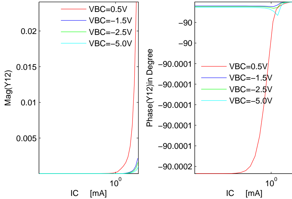
FIGURE 25. Y12 (extracted at 2.8GHz) vs IC(mA) plots at T=300K for Vbc=0.5,-1.5,-2.5, and -5V with collector current spreading effect.
