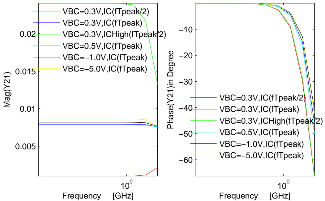
FIGURE 62. Y21 vs Frequency(GHz) plots at T=300K, Vbc=0.3, 0.5, -1.0 and -5.0V for IC(fTpeak),IC(ftpeak/2)and ICHigh(fTpeak/2).
