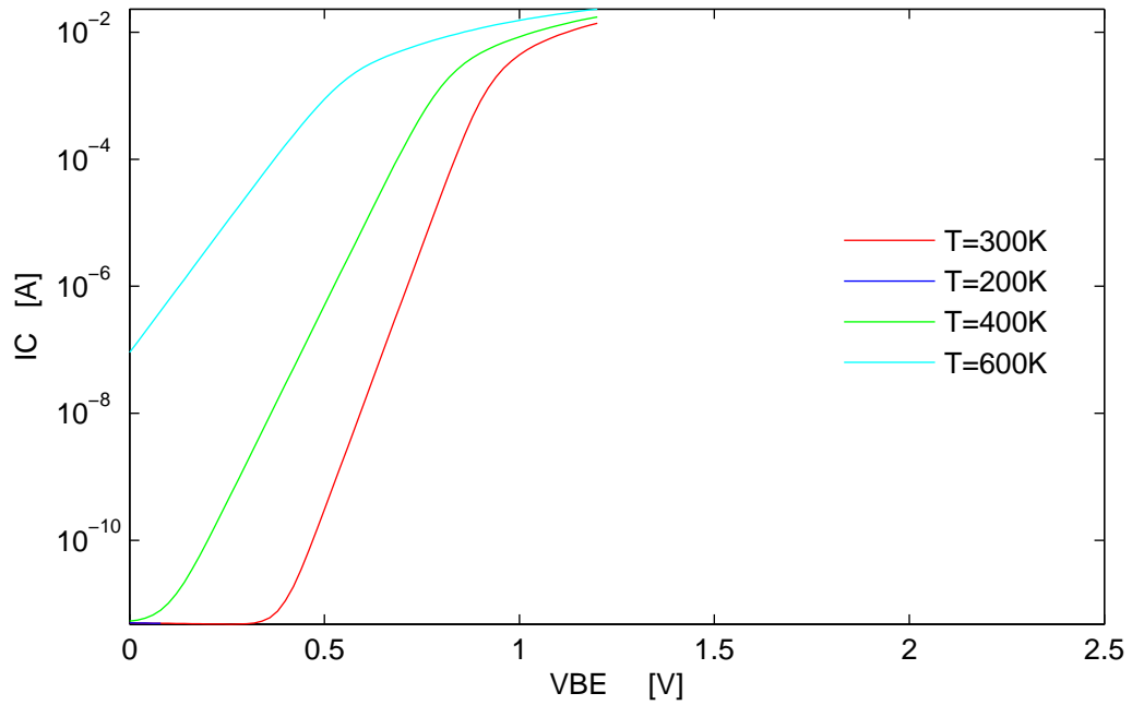
FIGURE 82. I_C vs. V_{BE} at V_{CE}=2.5\text{V} and T=200\text{K}, 300\text{K}, 400\text{K}, 600\text{K} .
