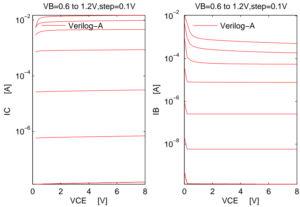
FIGURE 53. Forced-VB output characteristics and I_b -VCE plots at T=300K .
