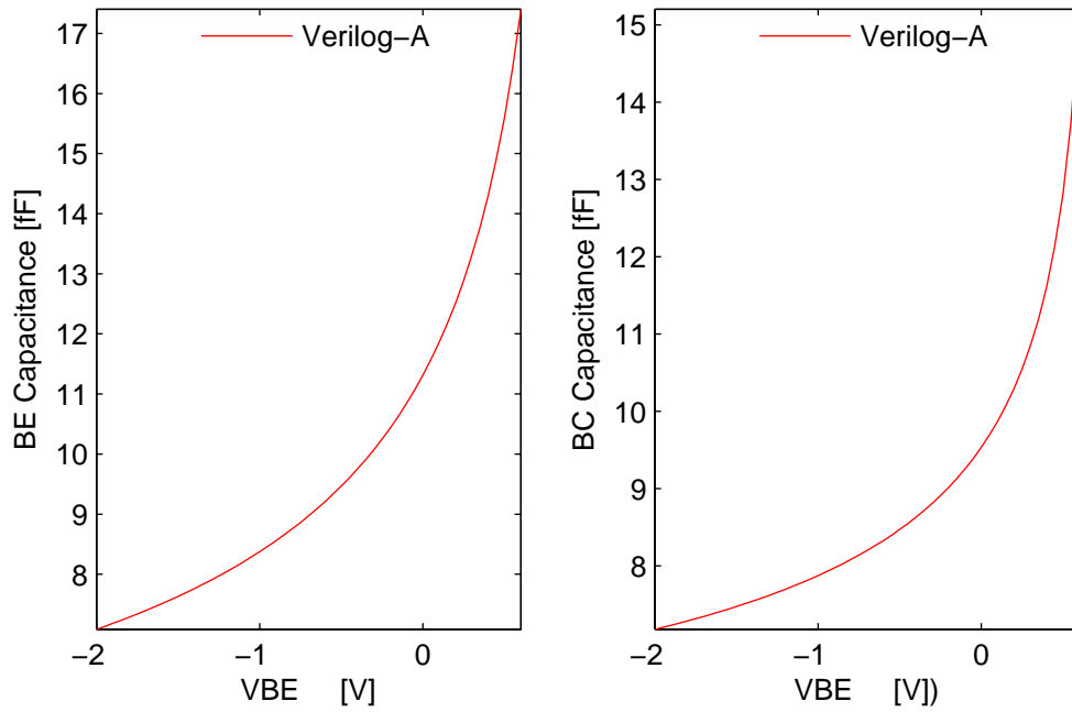
FIGURE 81. Depletion capacitances, C_{be} and C_{bc} (fF) vs BE voltages (Volt) plots at T=300\text{K} with collector current spreading effect.
