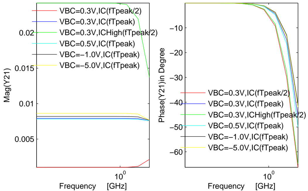
FIGURE 78. Y21 vs Frequency(GHz) plots at T=300K, Vbc=0.3, 0.5, -1.0 and -5.0V for IC(fTpeak),IC(ftpeak/2)and ICHigh(fTpeak/2) with collector current spreading effect.
