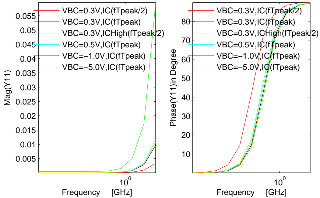
FIGURE 27. Y11 vs Frequency(GHz) plots at T=300K, Vbc=0.3, 0.5, -1.0 and -5.0V for IC(fTpeak),IC(ftpeak/2)and ICHigh(fTpeak/2) with collector current spreading effect.
