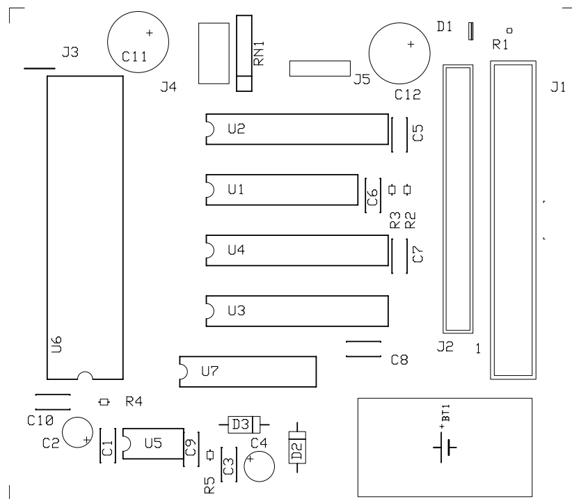
Figure 4: Component placement
